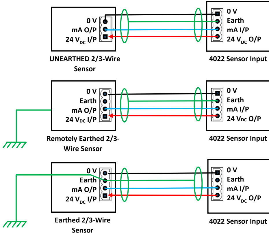
Figure 12: Connecting an a) unearth, b) remotely earth sensor to the 4022 or c) remotely earthed sensor.
